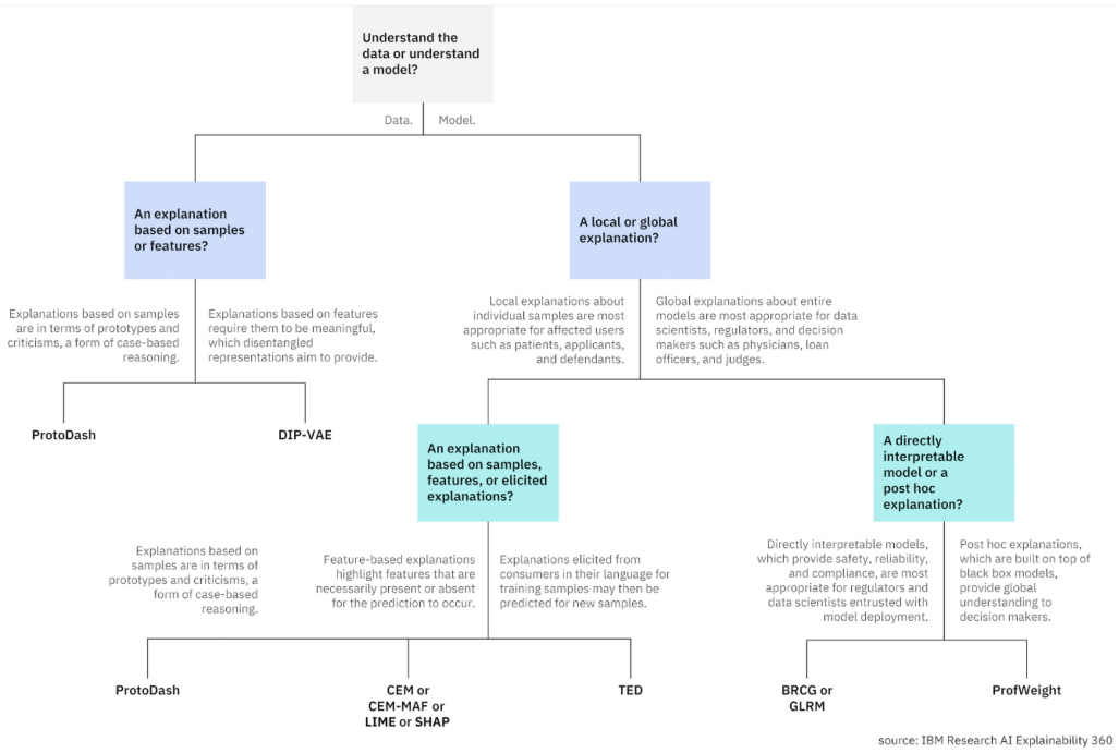
Fig. 5. Decision tree for AIX360 [63].
