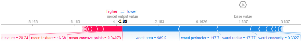
Fig. 13. Example: output of a SHAP plot.
