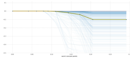
Fig. 8. An example of an ICE plot.
