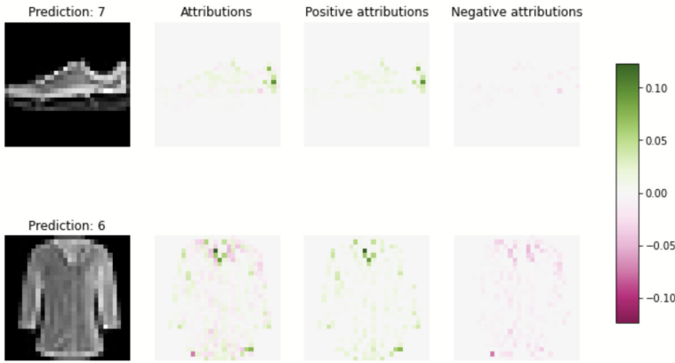
Fig. 20. An example of integrated gradients using the Fashion MNIST dataset.
