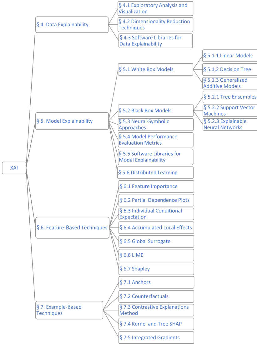
Fig. 3. A taxonomy of XAI techniques applies to data and the model.
