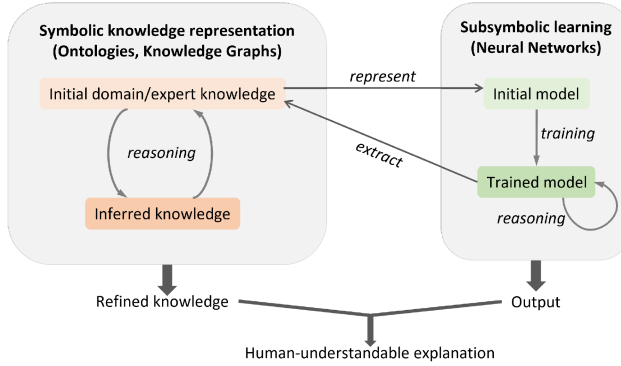
Fig. 4. High-level view of a neural-symbolic system [3].
